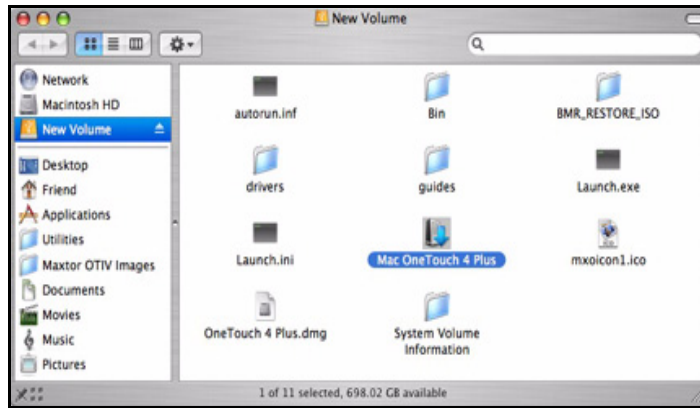
Figure 1: New Volume
