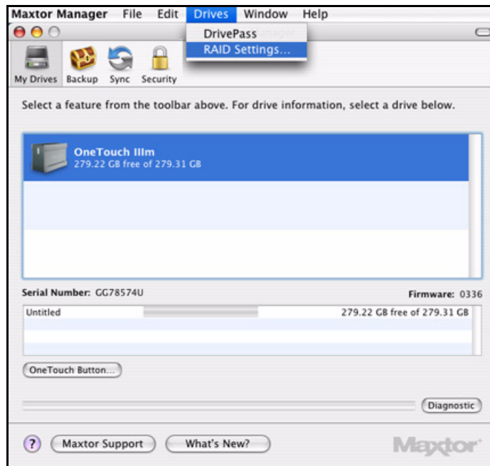
Figure 8: RAID Settings
