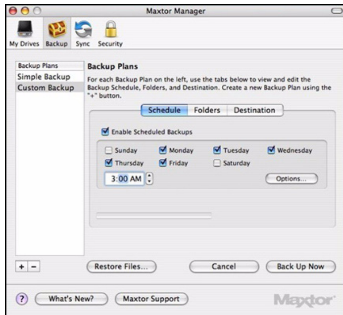
Figure 23: Backup Plans
