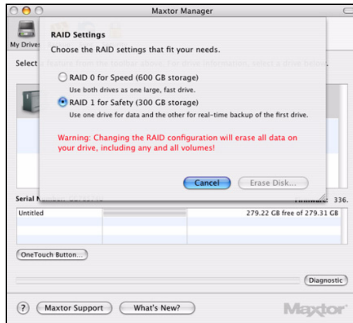
Figure 9: RAID Settings
