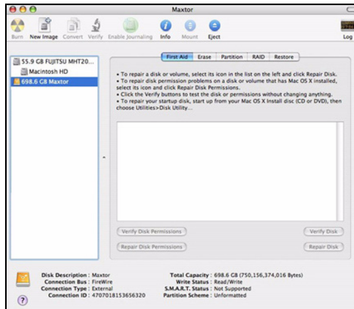
Figure 17: Disk Utility
