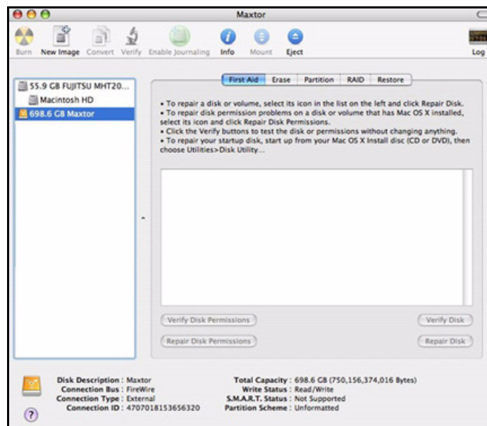
Figure 13: Disk Utility
