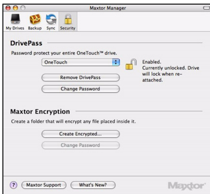
Figure 3: DrivePass Enabled
