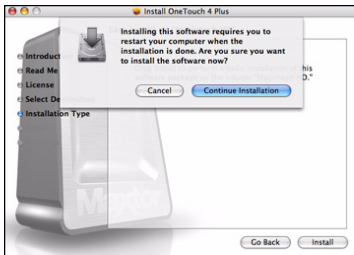
Figure 19: Restart Warning
