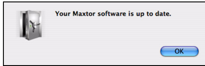
Figure 19: Software Update
