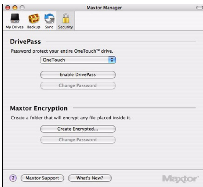
Figure 11: Security
